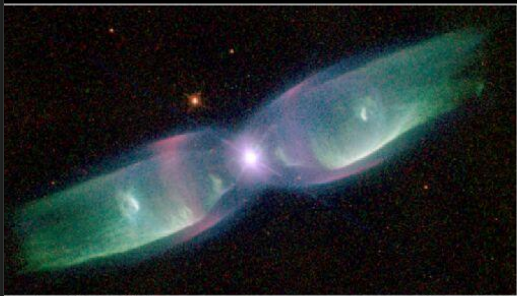
Planetary Nebula M2-9 RC97-38a • ST ScI OPO • December 17, 1997 J. Balick (University of Washington) and NASA
