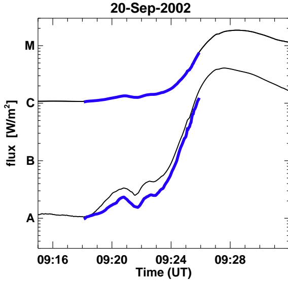
Fig. 4.— Comparison of the observed (black thin lines) and calculated (thick blue line) GOES fluxes in 1-8 Å (upper curves) and 0.5-4 Å (lower curves) energy bands during initial phase of the analyzed flare.
