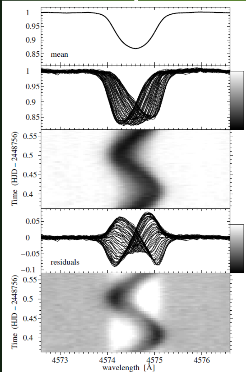
Fig. 2. An example of one night of data, in the wavelength range around the Si III \lambda 4574 line. From top to bottom: the mean of all 620 spectra — 54 normalized spectra taken on JD 2448756 — a grey-scale representation of the intensity variations in the line — the 54 residual spectra (mean spectrum subtracted from the normalized ones) — a grey-scale image of the residual intensity variations in the line
